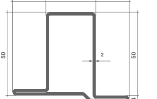
TD30-50x20x2 • 45%
