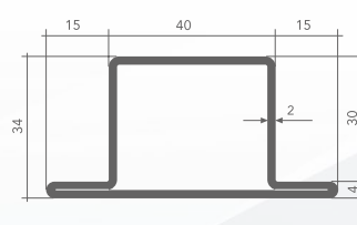
T40x34x15x2 • 50%
