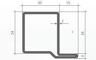
LD30-34x15x2 • 55%
