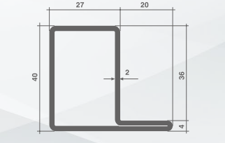
L27-40x20x2 • 50%
