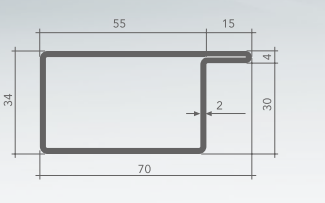
L55-34x15x2 • 40%
