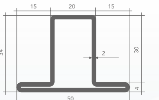
T20-34x15x2 • 60%
