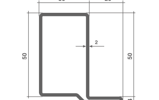
LD30-50x20x2 • 45%
