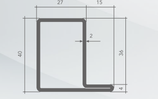
L27-40x15x2 • 50%
