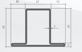
T27-40x15x2 • 50%
